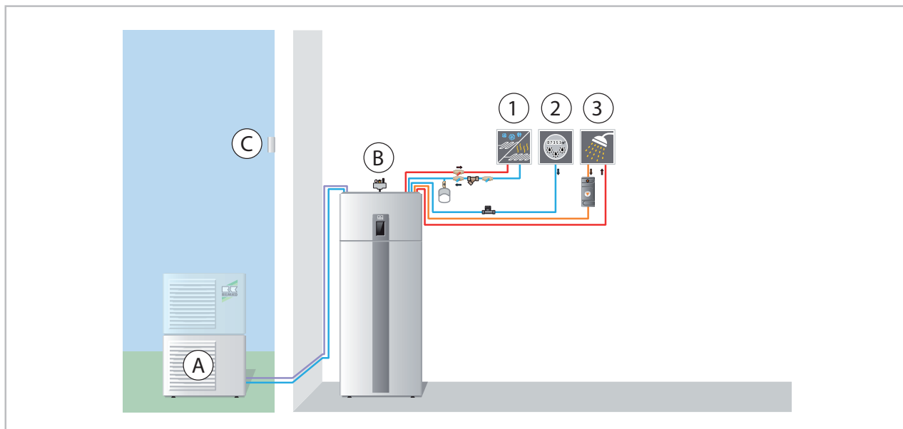
Fig. 76: Example hydraulic diagram WKF-compact
