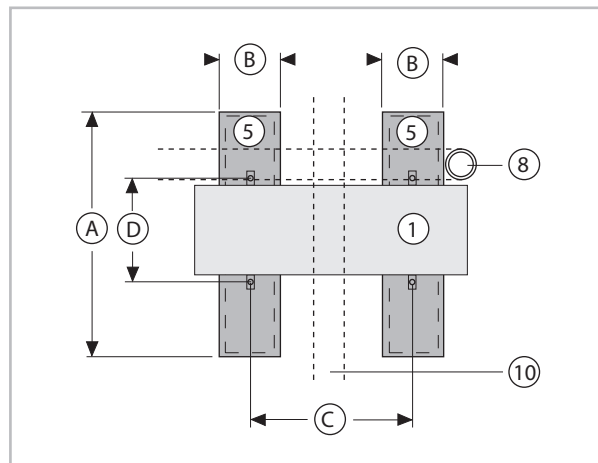
Fig. 73: Dimensions for the strip foundation (bird's eye view)
