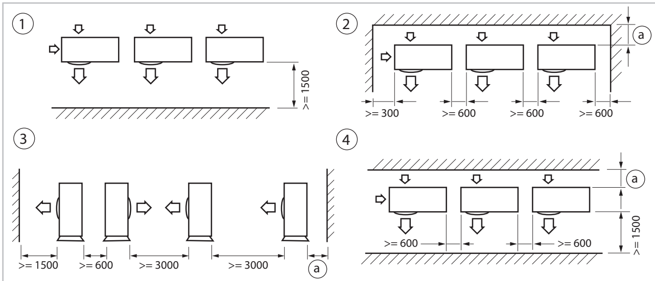
Fig. 71: Minimum distances during construction of multiple outdoor units in mm
