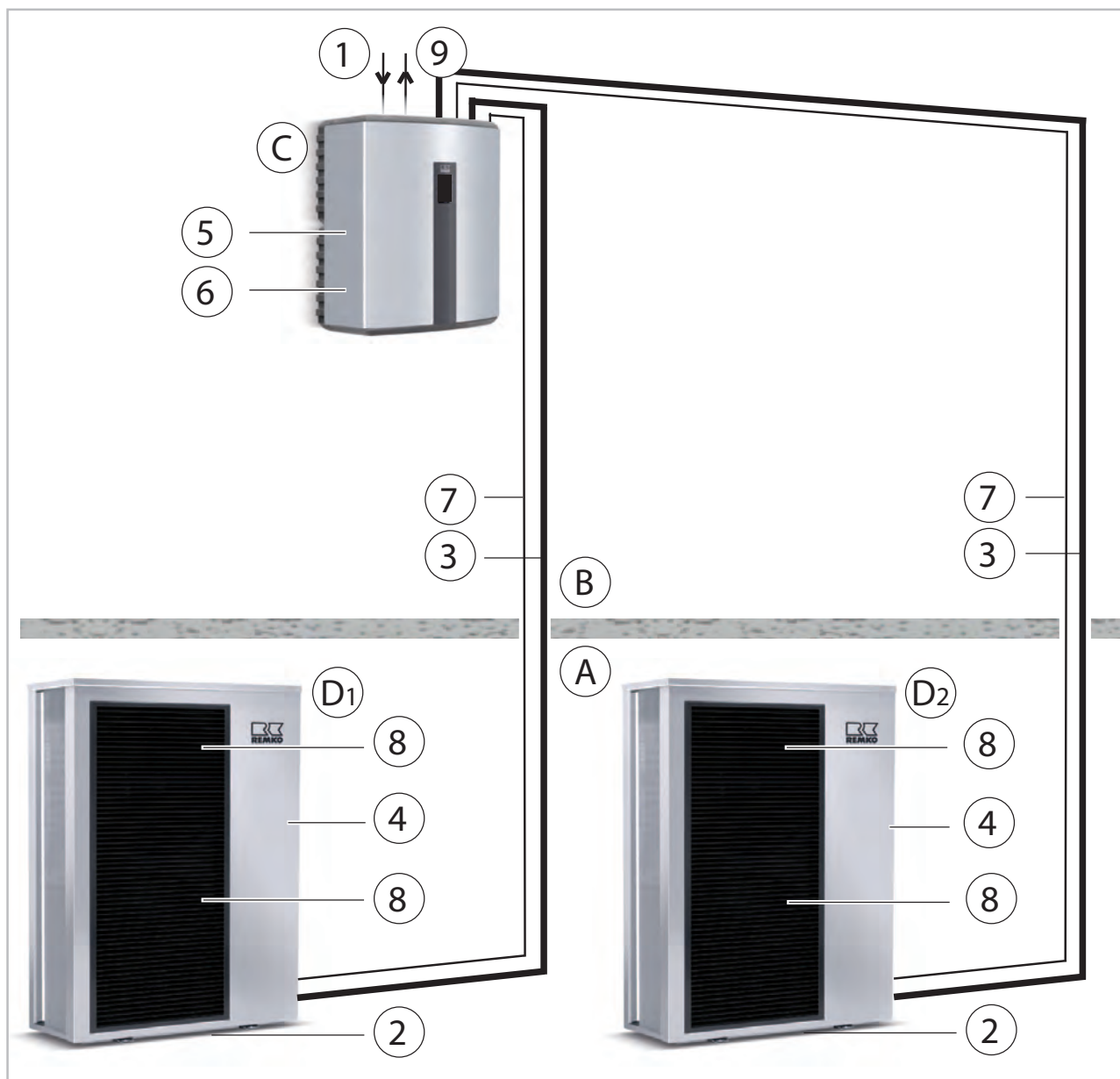
Fig. 61: System layout
