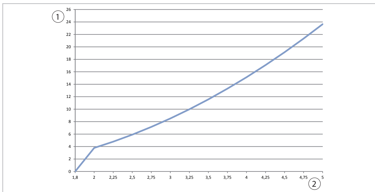
Fig. 63: Minimum space for unventilated installation rooms based on fill quantity with an installation height of 1.6 m
