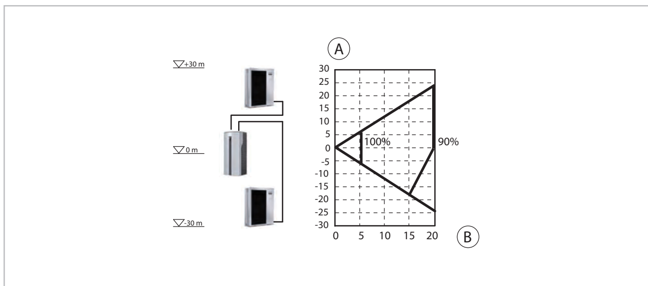
Fig. 51: Cooling output losses at WKF/ WKF-compact 170/WKF 170 Duo
