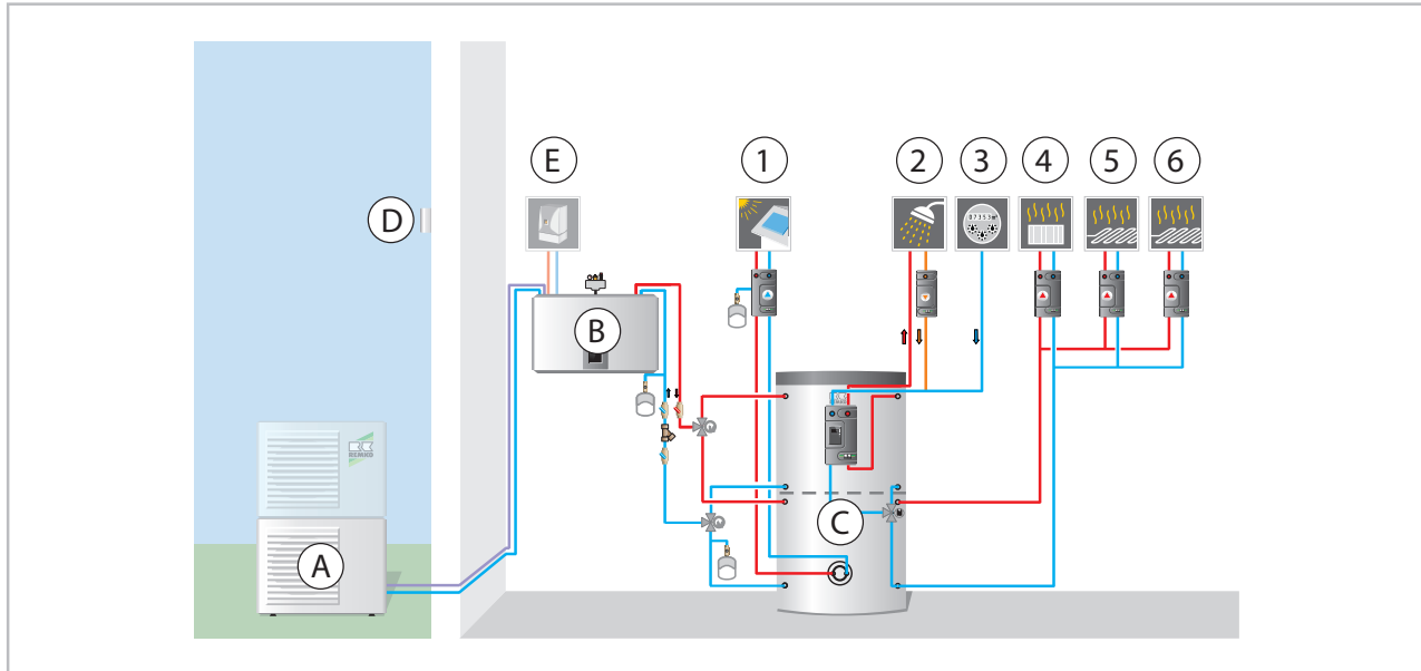
Fig. 75: Example hydraulic diagram WKF
