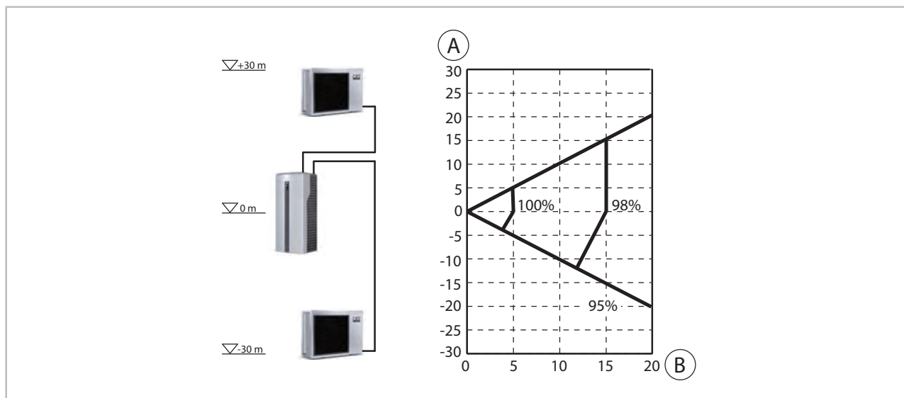
Fig. 45: Cooling output losses at WKF/WKF-compact 80
