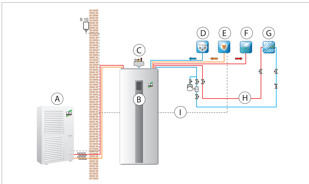
Fig. 67: Safety assembly – Installation schematic
