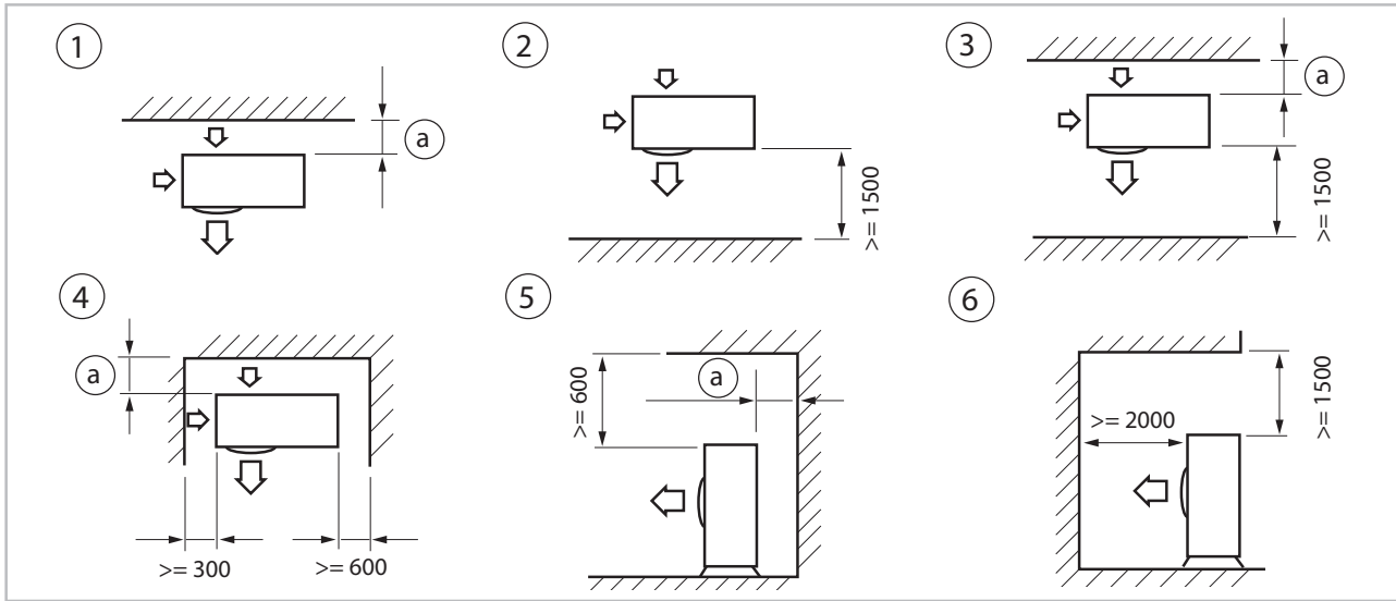
Fig. 70: Minimum distances during construction of an outdoor units in mm
