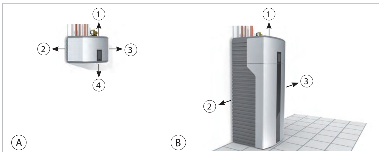
Fig. 66: Minimum spacing for indoor units
