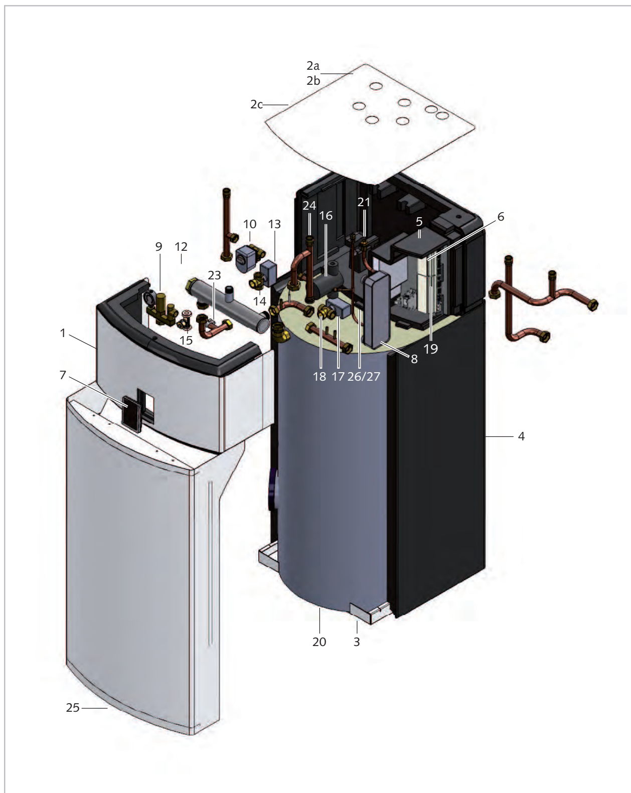
Fig. 85: Exploded view
