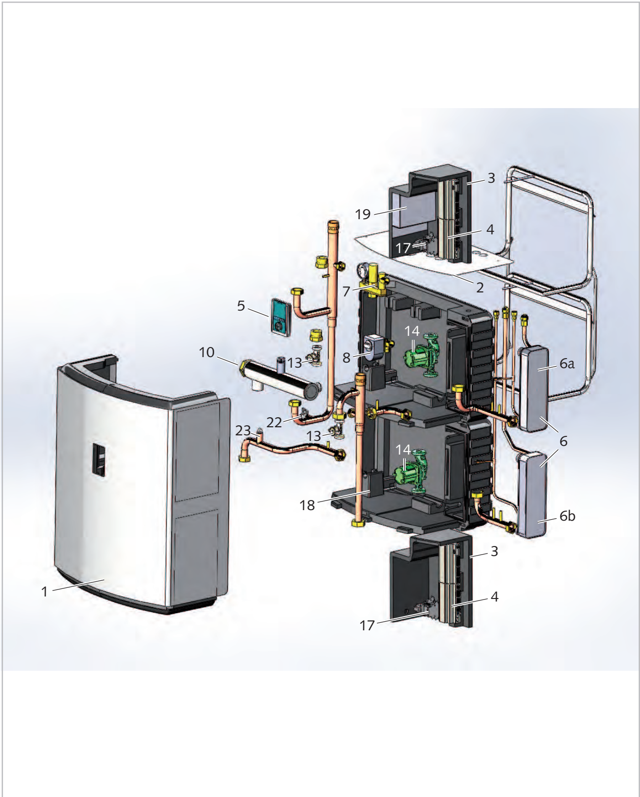
Fig. 86: Exploded view
