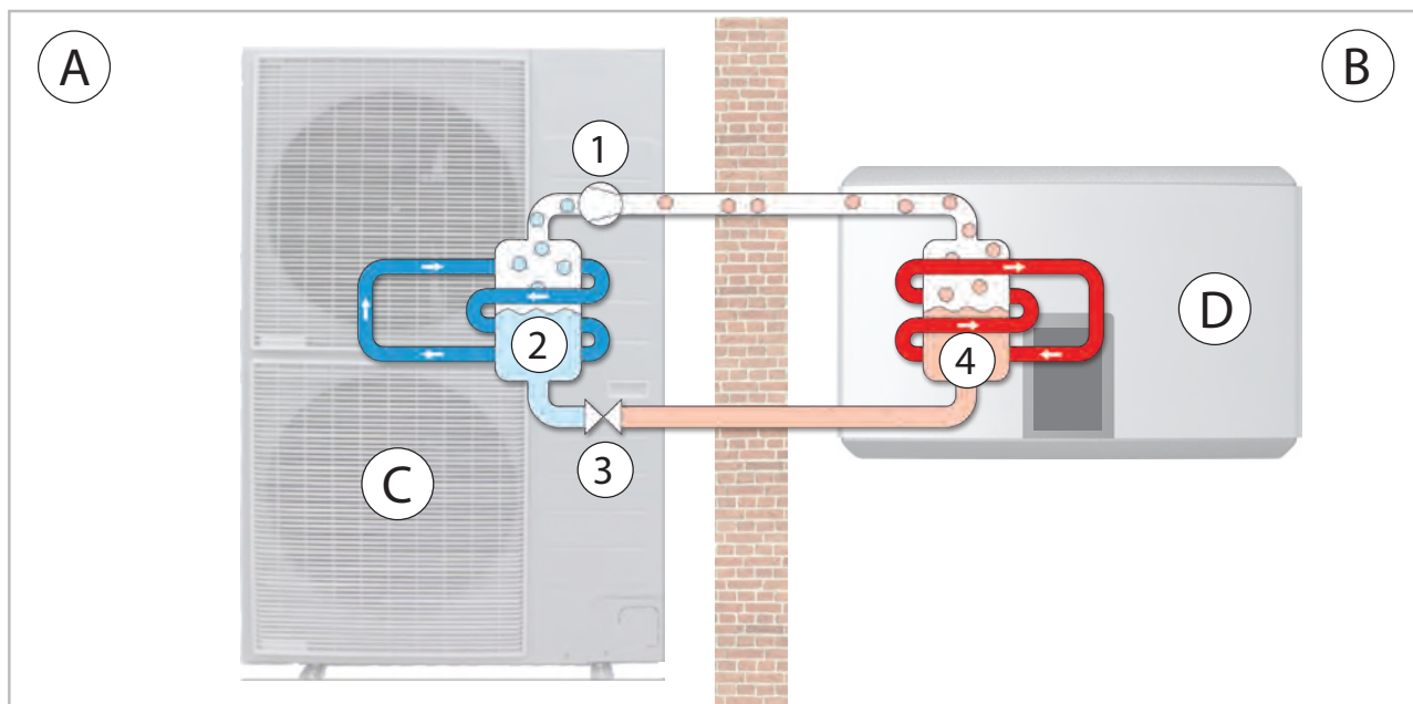
Fig. 53: Functional diagram heating inverter heat pump
