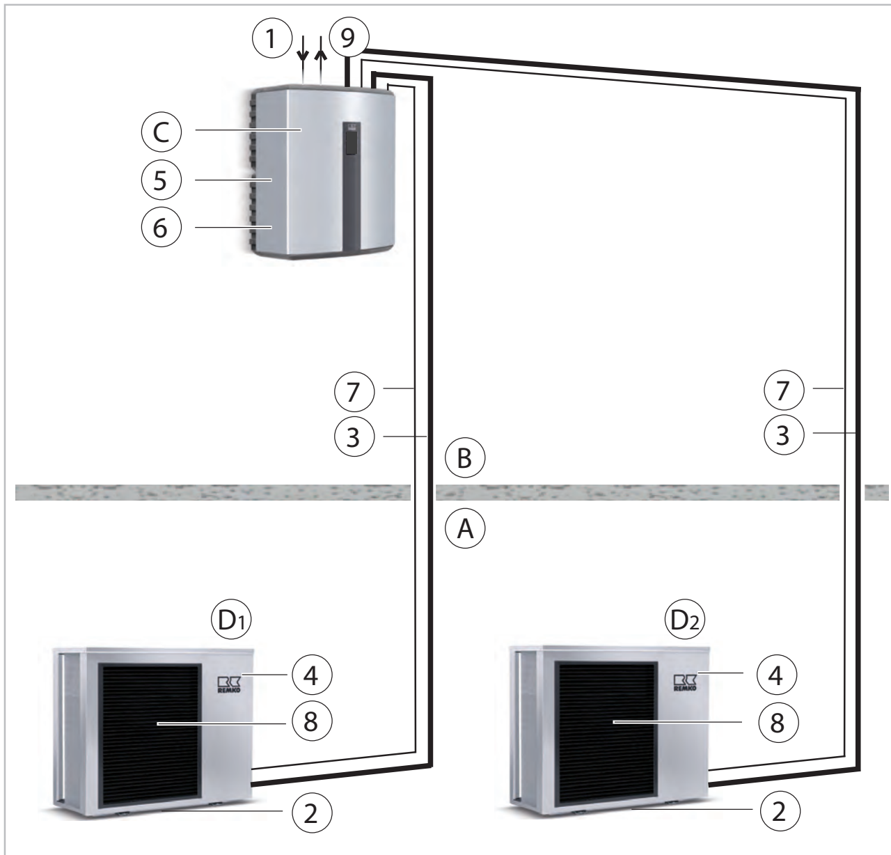
Fig. 60: System layout
