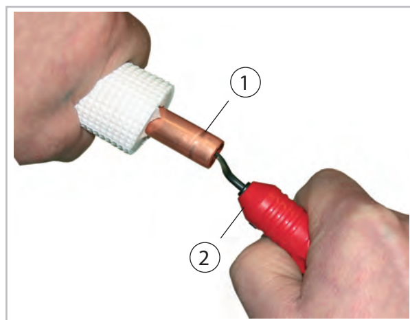
Fig. 78: Deburring the refrigerant piping
