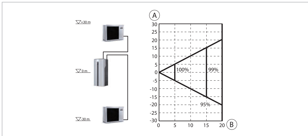
Fig. 44: Heat output losses at WKF/WKF-compact 80
