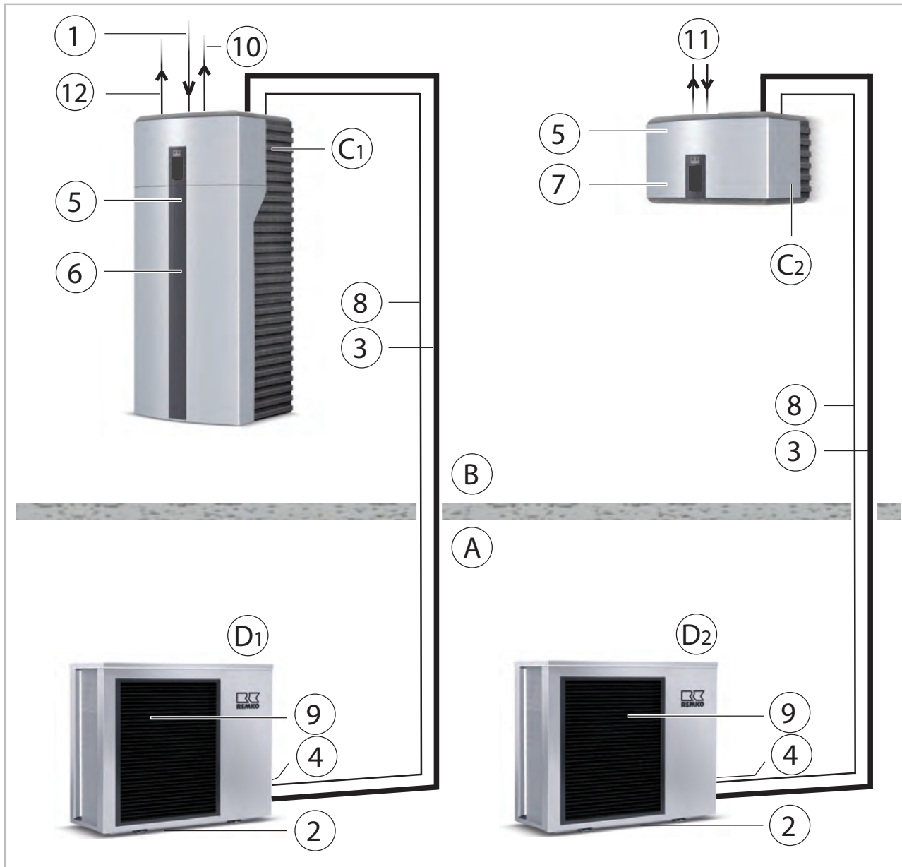
Fig. 58: System layout
