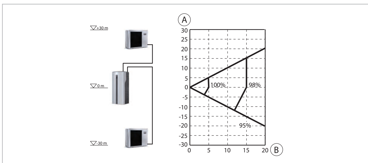
Fig. 47: Cooling output losses at WKF/WKF-compact 100
