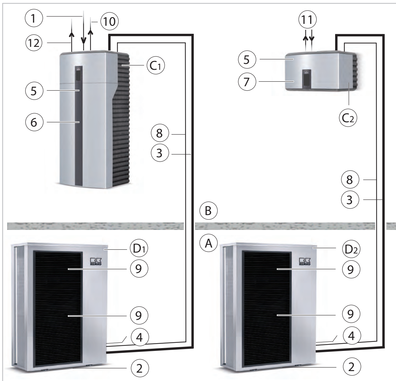
Fig. 59: System layout
