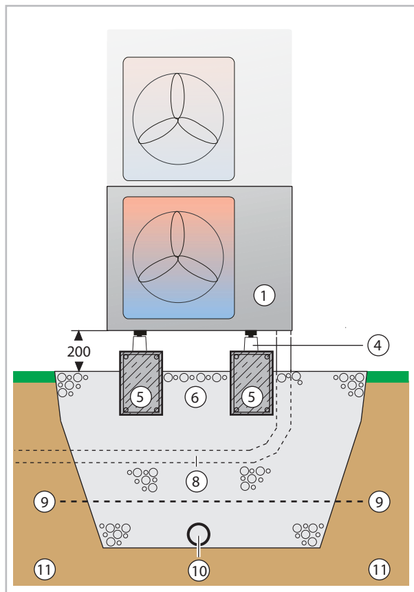
Fig. 72: Condensate drainage, seepage of condensate and strip foundation (cross-section)
