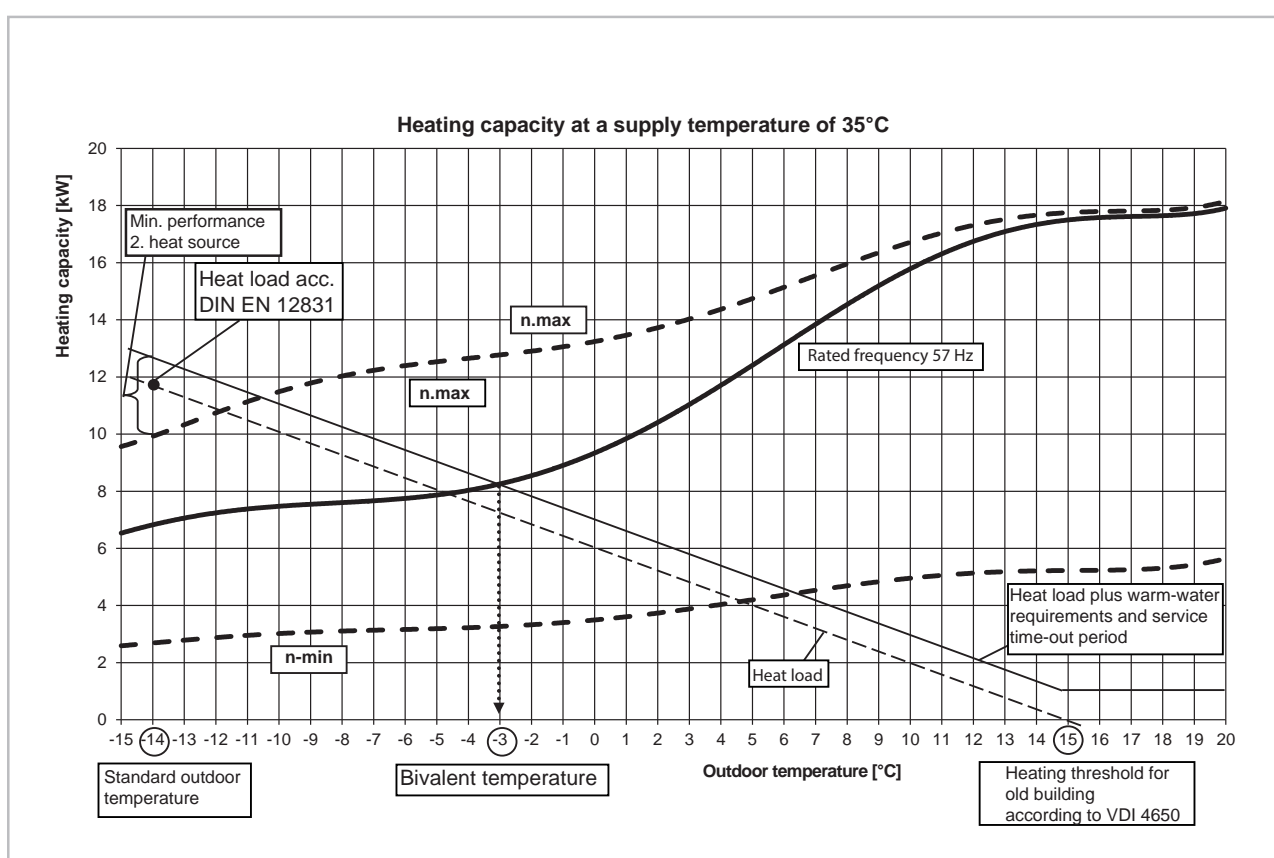
Fig. 54: Heating capacity diagramm of the heat pump WKF/WKF-compact 170
