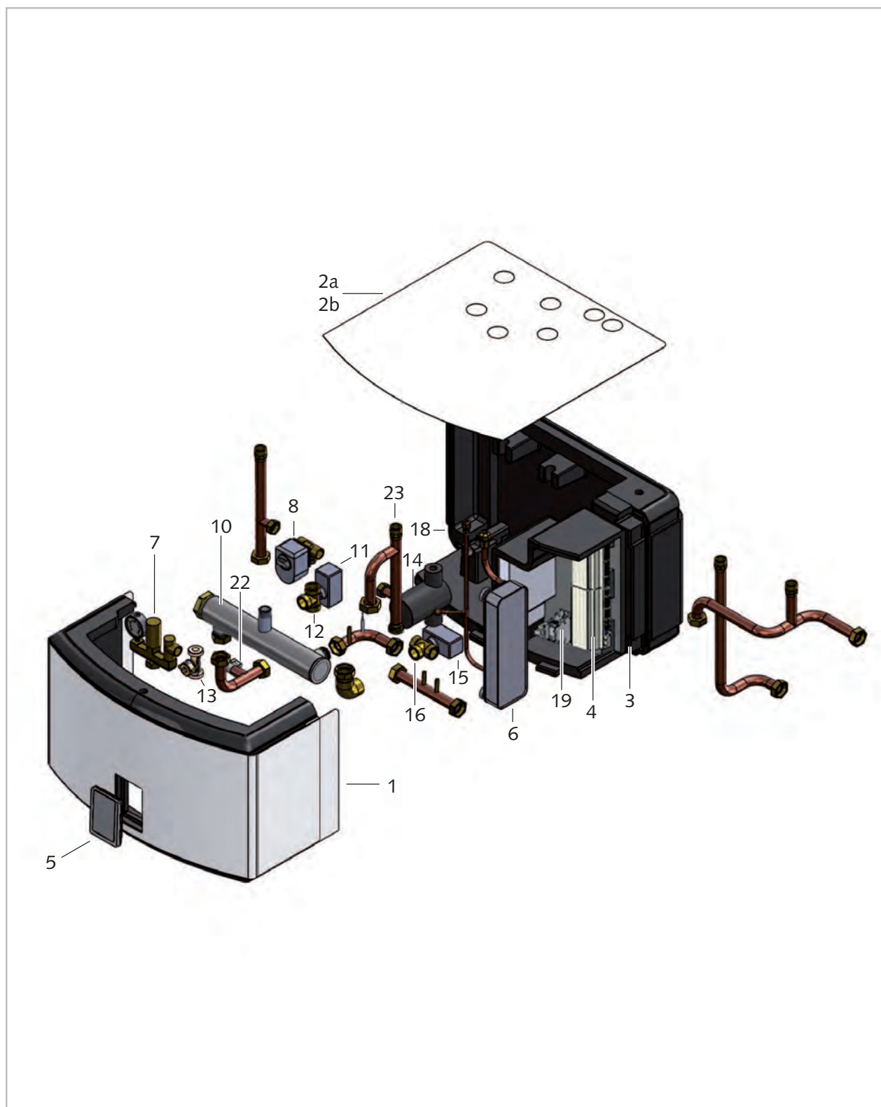
Fig. 84: Exploded view
