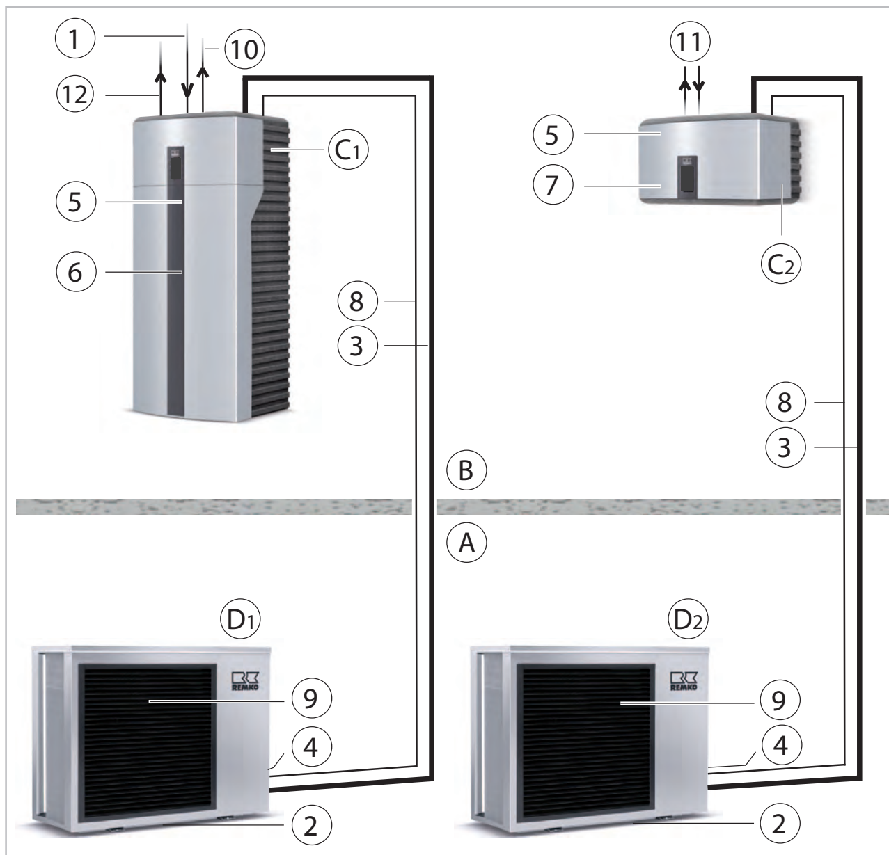
Fig. 57: System layout
