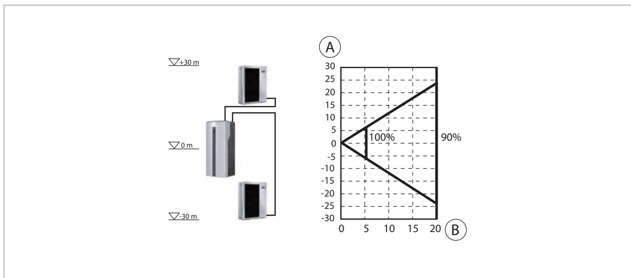
Fig. 50: Heat output losses at WKF/WKF-compact 170/WKF 170 Duo
