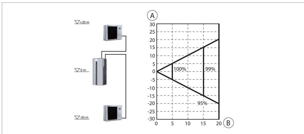
Fig. 46: Heat output losses at WKF/WKF-compact 100
